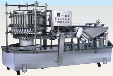
棒棒冰充填封口機 Ice Tube (Bong-Bong Ice) Filling & Sealing Machine
